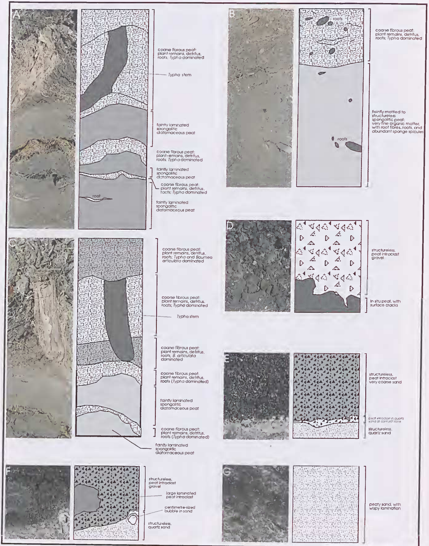
Figure 5. Annotated cores of selected sediments (width of all cores is 10 cm). A–C. Cores of peat. D–G. Cores of peat intraclast gravel and sand, quartz sand, and peaty sand. H–K. Cores of calclutite, and carbonate intraclast gravel and sand. L–M. Cores of diatomite, and diatomite intraclast gravel.
